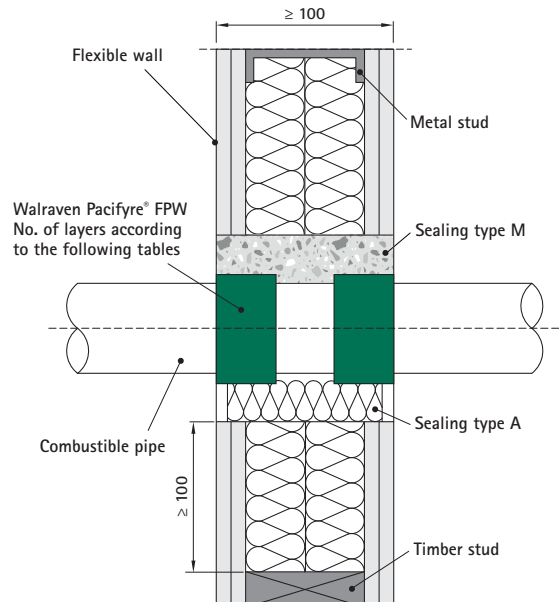
Double-sided flexible wall construction type b)
