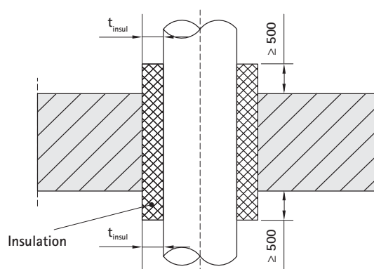
Local sustained insulation (LS)
